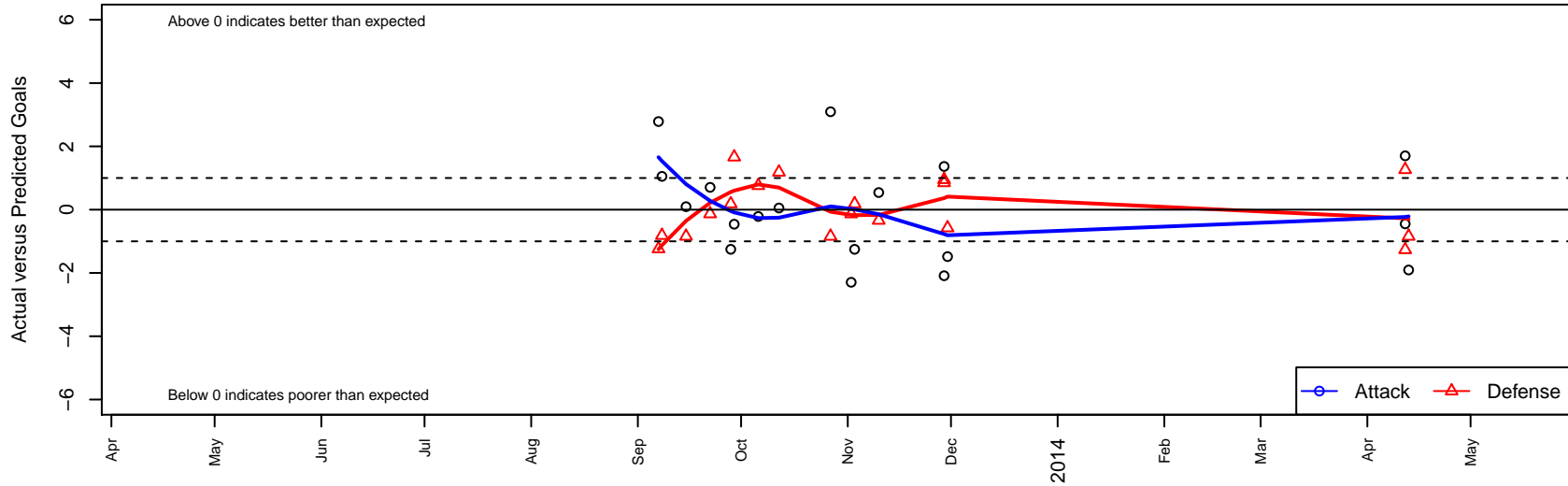
Foothill Storm SC B96 Dots are actual minus expected GF (blue circles) and GA (red triangles). Blue line is smoothed change in attack strength. Red is smoothed change in defense strength.
